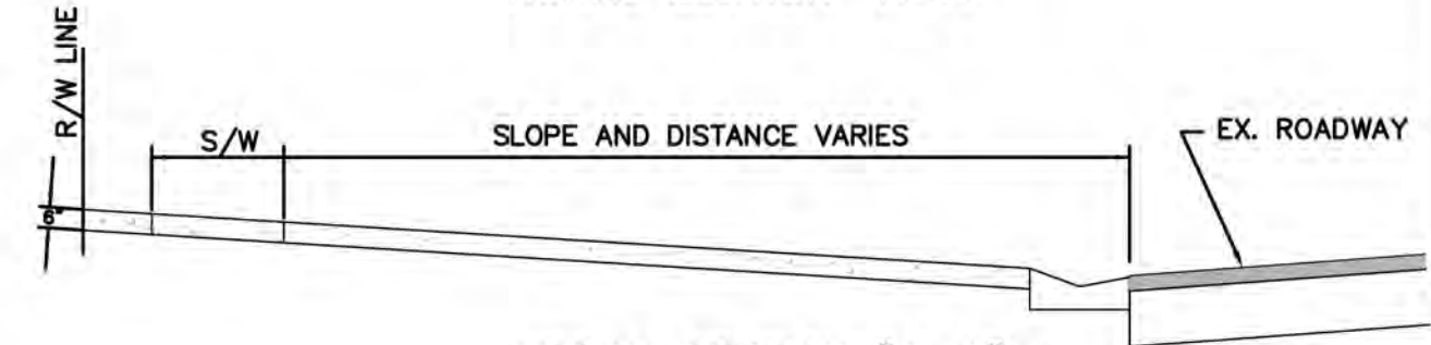
URBAN SECTION "A-A"
