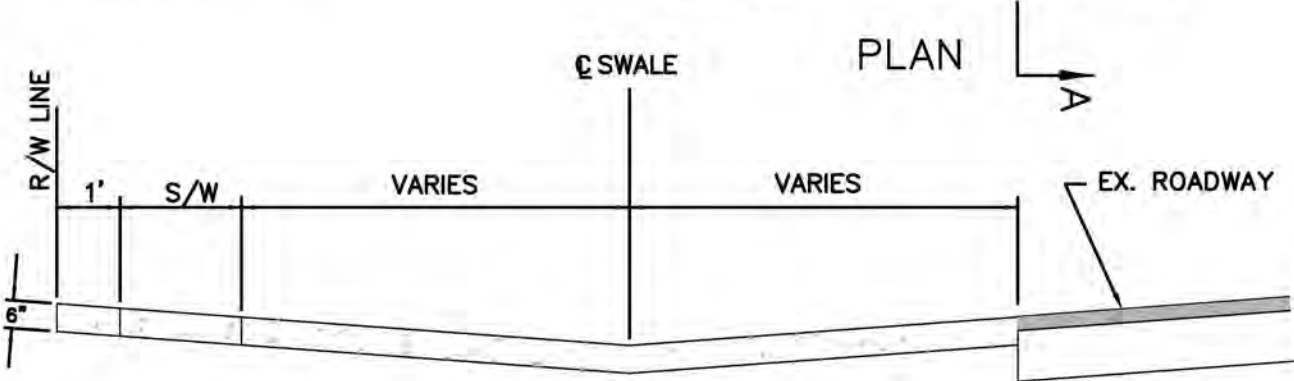
RURAL SECTION "A-A"
